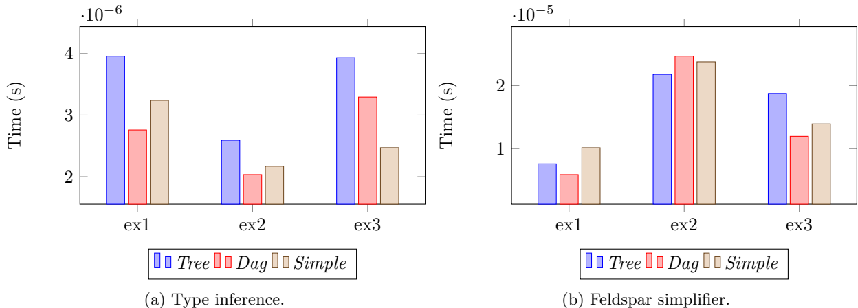
Figure 15: Benchmark: type inference and Feldspar simplifier.
