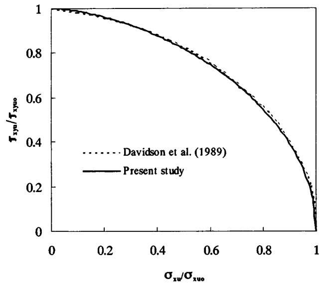
Fig. 11. Comparison of present study with existing results for plate with b/t=40 , a/b=1 , \alpha=1
