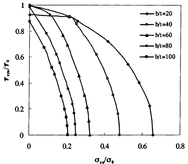
Fig. 8. Strength interaction curves of plates with various b/t ratios, a/b = 1, \alpha = 1
