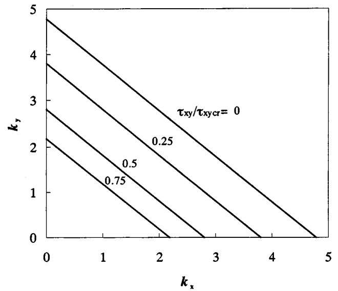
Fig. 5. Buckling interaction curves of plates under constant shear stresses (S-S-S-S+SC), a/b = 1 , \alpha = 1
