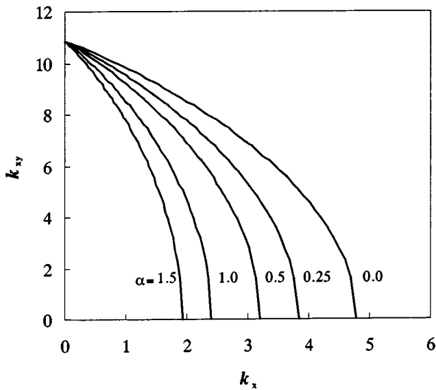
Fig. 4. Buckling interaction curves of plates (S-S-S-S+SC), a/b = 1
