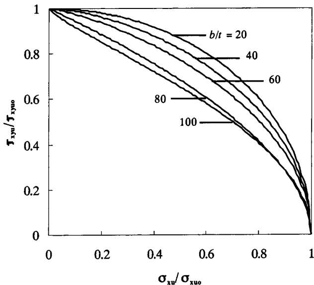
Fig. 10. Strength interaction curves of plates by proposed design models, a/b=1 , \alpha=1
