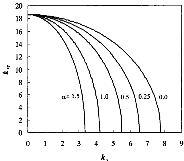
Fig. 7. Buckling interaction curves of plates (C-C-S-S+SC), a/b = 1
