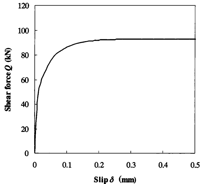
Fig. 3. Shear–slip curve for stud shear connectors
