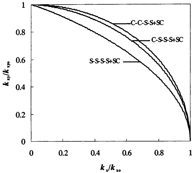
Fig. 9. Normalized buckling interaction curves of plates with different boundary conditions, a/b=1
