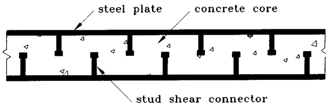
Fig. 1. Cross section of double skin composite panel
