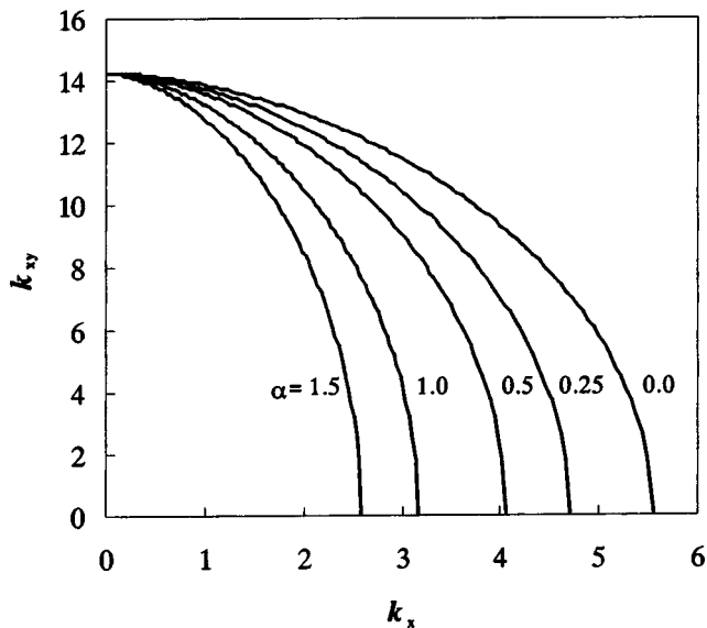
Fig. 6. Buckling interaction curves of plates (C-S-S-S+SC), a/b = 1
