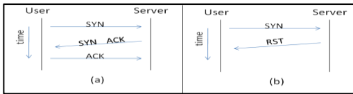
Figure 6. TCP 3-way handshake. (a) The 3-way handshake with an open port. (b) Connection attempt on a closed port.
