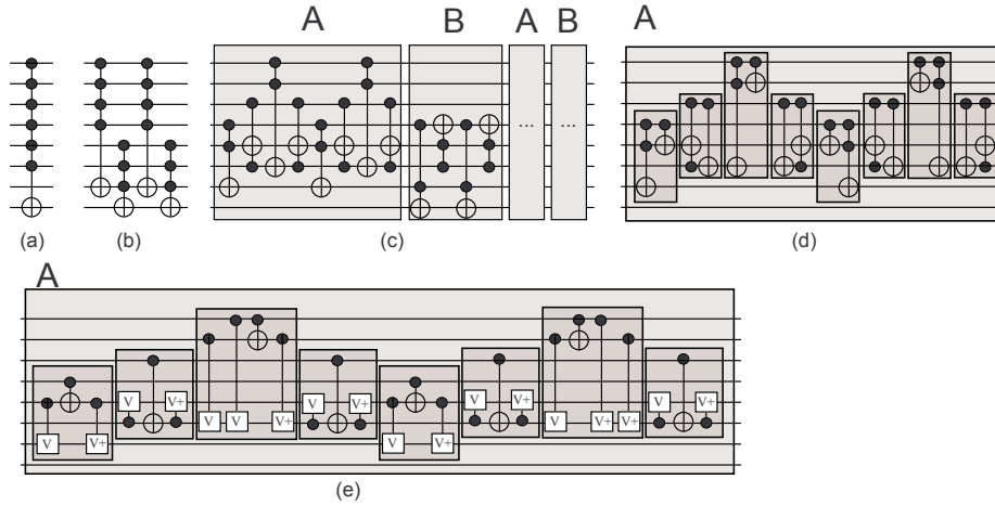
Fig. 9. Decomposition of a C^6\text{NOT}(a,b,c,d,e,f,h) gate into smaller multiple-control Toffoli gates [Barenco et al. 1995] (b) and Toffoli gates [Barenco et al. 1995] (c), Peres gates [Maslov and Dueck 2003] (d), elementary gates [Maslov et al. 2008a] (e), in the presence of one garbage line.
