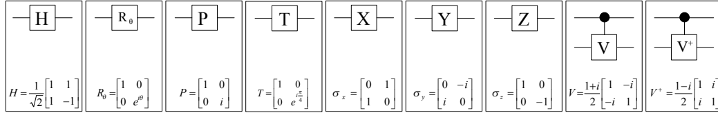
Fig. 5. Basic quantum gates: Hadamard, phase shift, Phase, \frac{\pi}{8} , Pauli-X (NOT), Pauli-Y, Pauli-Z, controlled-V, and controlled-V ^\dagger .
