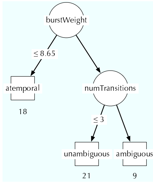
Fig. 15. Decision tree learned to classify queries in the web search log dataset (Table IV). Numbers under the leaf nodes represent number of class instances correctly labeled. Each class has 24 instances. Most of the temporally unambiguous and atemporal queries are correctly classified using only features of the burst model (burst weight and number of state transitions).
