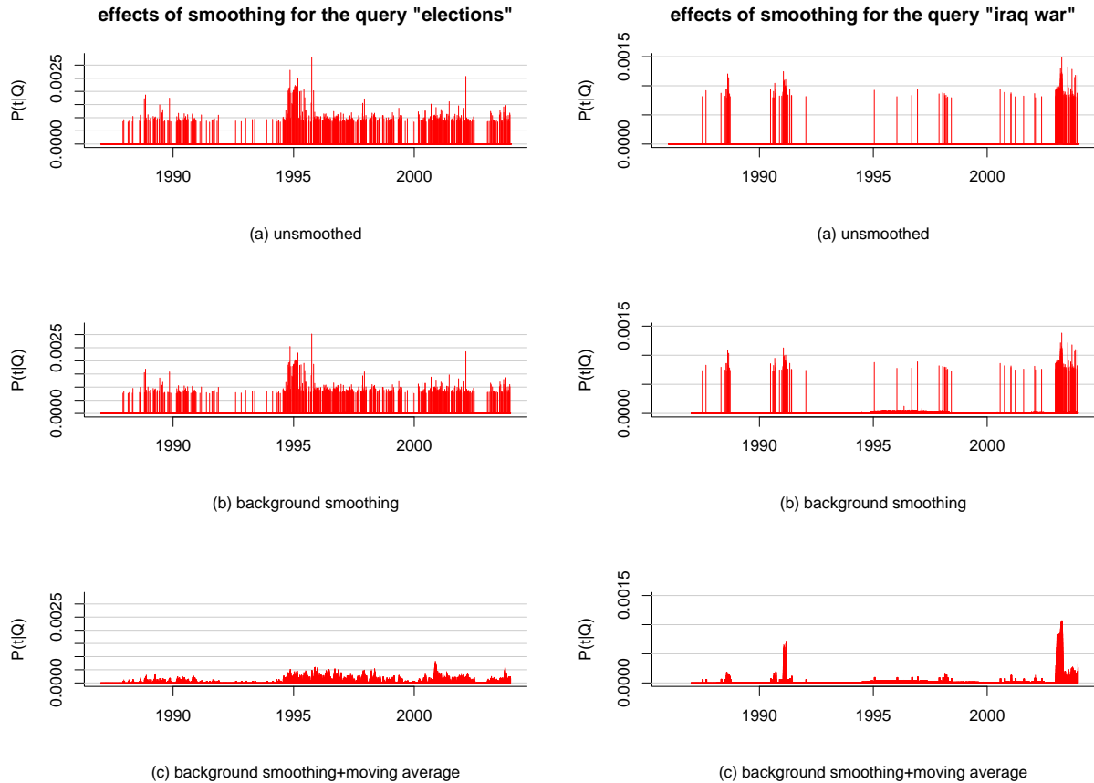
Fig. 3. Probability of relevance of each day, for the queries “elections” (left) and “iraq war” (right) on documents from 1986 through 2004
