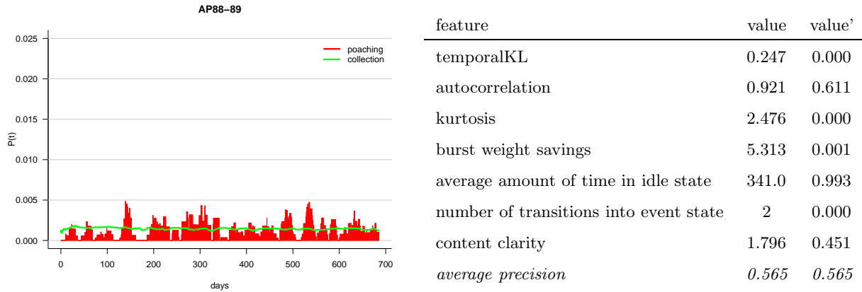
Fig. 10. Temporal profile and raw and normalized feature values for the query “Poaching” over the AP88-89 collection. We normalized feature values by shifting and scaling them to lie between zero and one. This query had the minimum score for both temporal KL and number of transitions into the event state, and so the scores for both of these features are zero after normalization.
