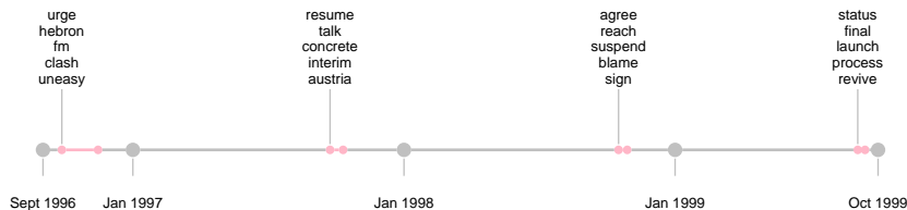
Fig. 16. Non-extracted Summaries: The AQUAINT corpus was used to visualize the temporal profile of the query “Israel-Palestine”. Kleinberg’s burst model is used to detect event boundaries. Event language models are built from documents within these ranges. Summaries consist of the terms with the highest point Kullback-Leibler divergence with respect to the collection language model.
