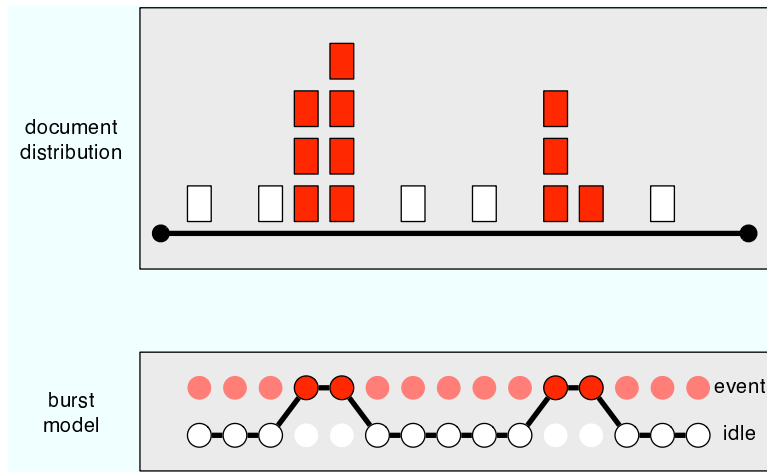
Fig. 6. The top frame shows the distribution of retrieved documents over the time span of the collection (one rectangle=one document). Documents highlighted in red provide evidence of an event or “burst”. The bottom frame shows a model of the burstiness of the distribution. The burst model considers each day in the time span as either being relevant to a burst (such a day is in the “event” state) or not relevant to a burst (such a day is in the “idle” state). The highlighted sequence of states represents a model of the transition between event and idle states over the course of the time span.
