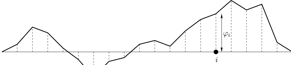
FIG 1. A one-dimensional interface \varphi .
