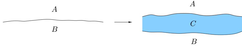
FIG 6. When \tau_{AB} > \tau_{AC} + \tau_{BC} , a layer of the equilibrium phase C is spontaneously created at the interface between the equilibrium phases A and B , thus giving rise to a problem of entropic repulsion between multiple interfaces.
