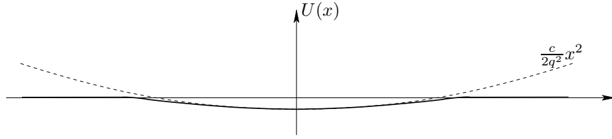
FIG 10. The pinning potential considered in [46] and its quadratic approximation yielding the effective mass.
