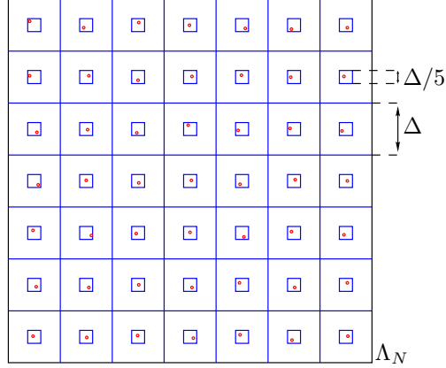
FIG 13. The box \Lambda_N is decomposed into cells of sidelength \Delta , in each of which a smaller cube of sidelength \Delta/5 is centered. The partition function is estimated by considering only configurations containing exactly one pinned point inside each of the smaller cubes.
