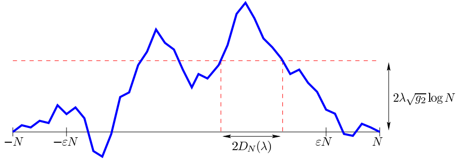
FIG 2. D_N(\lambda) measures the width of the widest spike reaching above 2\lambda\sqrt{g_2} \log N in the subbox \Lambda_{\varepsilon N} (of course, the real situation is 2-dimensional).
