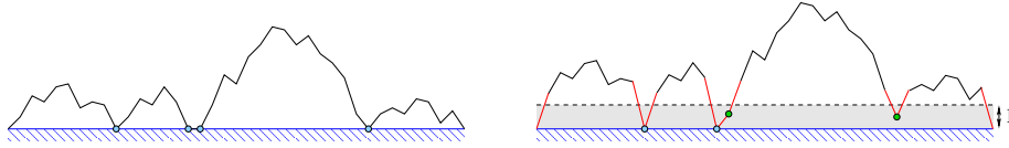
FIG 12. The transformation: A random subset of the pinned sites is unpinned and the height at the corresponding sites is chosen at random in the interval (0, 1) . To avoid overcounting, the whole interface, except the pinned sites, is lifted by 1 before this procedure is applied.
