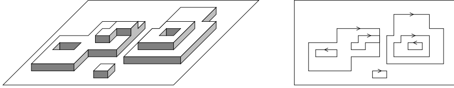
FIG 4. The oriented level lines of a discrete effective interface; the orientation specify the type of the contour, i.e. whether it is increasing or decreasing the surface height. For convex interactions V , the resulting contours satisfy a Peierls estimate and are therefore amenable to a rigorous study through perturbative arguments.
