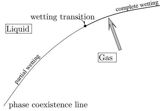
FIG 15. How does the width of the layer of unstable phase diverges as the coexistence line is approached, in the regime of parameters where complete wetting occurs?
