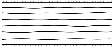
FIG 7. A stack of interfaces between two fixed walls. Another variant consist in an infinite “one-dimensional” gas of d -dimensional interfaces with positive fugacity.
