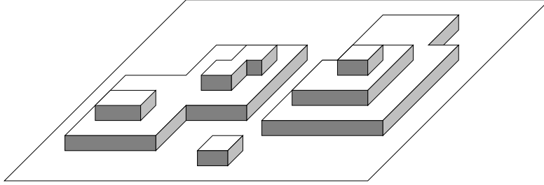
FIG 5. A picture of the wedding cake model. Gradients can take only values 0 and \pm 1 , and the interface height can only increase. The level lines of this model are exactly identical to the contours of the two-dimensional Ising model.
