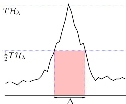
FIG 16. Idea behind the proof of the tail exponent.
