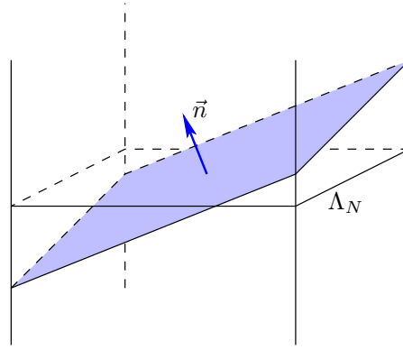
FIG 3. A sketch of the cylinder \Lambda_N \times \mathbb{Z} and the associated tilted boundary condition \psi_{\vec{n}} .
