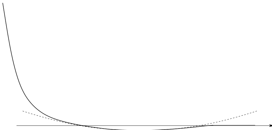
FIG 14. A sketch of the type of potential considered in [46, 78]. The hard wall is replaced by a fast growth, the pinning part is very shallow, very wide, and very well approximated by a parabola, the curvature of which yields the effective mass of the system.
