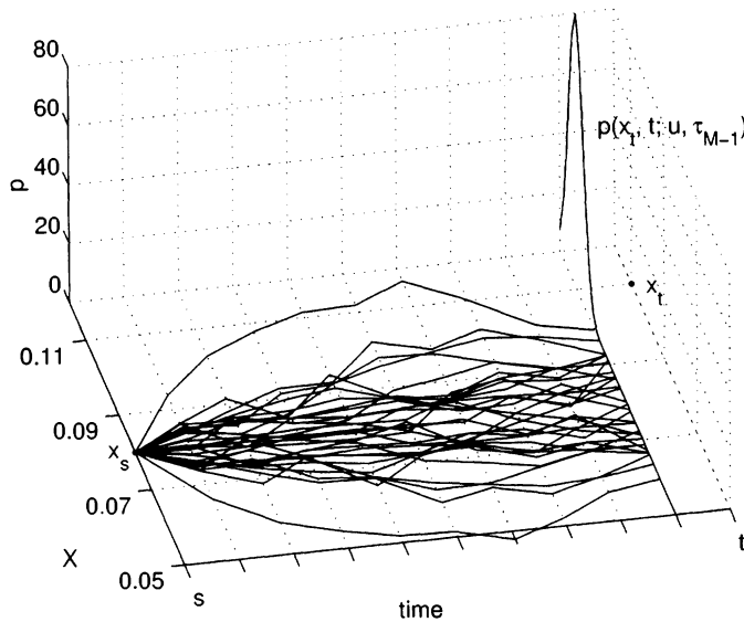
Figure 4. Illustration of Equation (16). The terminal points of the sample paths represent draws from P_{M-1}^{(M)} ; the curve represents the integral.
