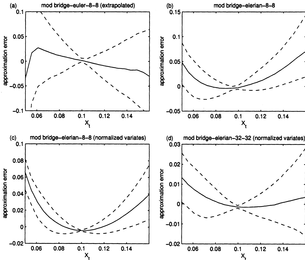
Figure 7. Approximation Error, \log \hat{p}(X_t, t; X_s, s) - \log p(X_t, t; X_s, s) , for Various Simulated Likelihood Schemes Given \Delta = t - s = 1/12 , X_s = .10 , and \theta = (.5, .06, .15) . The median and interquartile range over 128 repetitions are plotted. The untransformed model is used.
