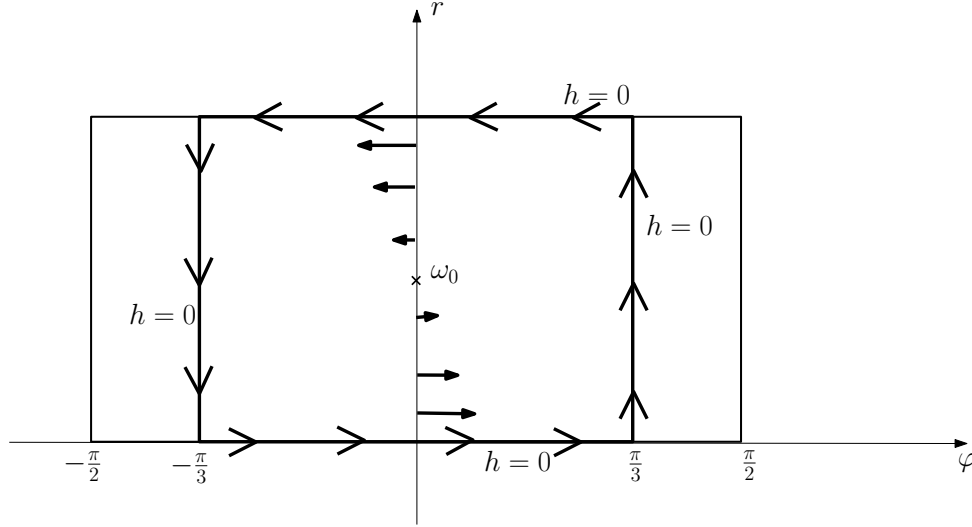
FIGURE 1. Phase diagram for h(\varphi, r)
