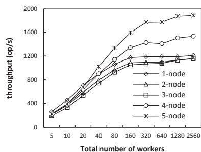
Figure 12: Results of the scalability test in Setup-SAS under workload B.
