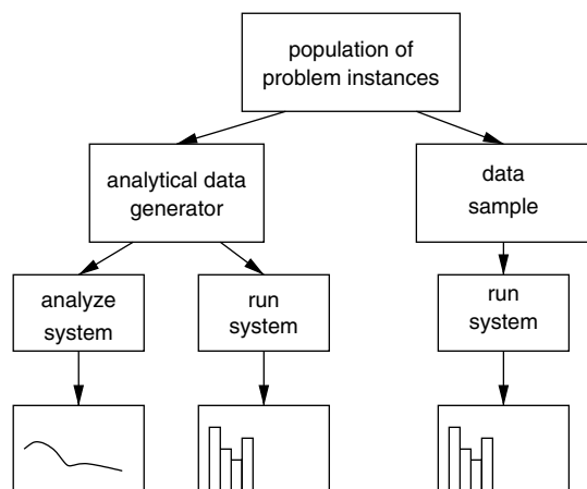
Fig. 1. Different approaches to validating algorithms.
