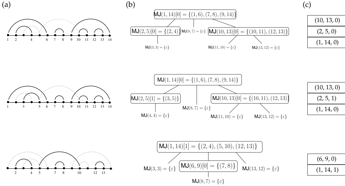
Figure 3: (a) Locally optimal secondary structures of Figure 2. (b) Associated ordered trees. MJ(i, j)[k] denotes the k th element of MJ(i, j) . (c) Content of the stack at the end of each iteration of the algorithm of Figure 4 (lines 5, 6 and 7). MJ(i, j)[k] is symbolized by the triplet (i, j, k) . Each cell of the stack corresponds to an internal node of the underlying tree depicted in (b). For example, at iteration 1, the line 5 pushes the triplet (1, 14, 0) , corresponding to MJ(1, 14)[0] = \{(1, 6), (7, 8), (9, 14)\} , then the nested structures are pushed.
