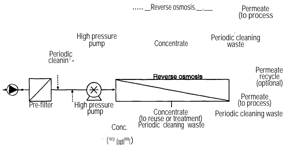
Figure 4-2. Reverse osmosis system.
