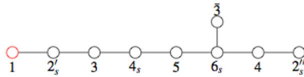
Fig. 1. McKay correspondence for E_8 and 2I : Dynkin diagram for the standard affine extension of E_8 , here denoted E_8^+ , and the graph for the tensor product structure of the binary icosahedral group 2I , where nodes correspond to irreducible representations (labelled by their dimension d_i , and a subscript s denotes a spinorial representation). The affine root \alpha_0 of E_8^+ (red) corresponds to the trivial representation of 2I and is given in terms of the other roots as -\alpha_0 = \sum d_i \alpha_i . The sum of the dimensions of the irreducible representations of 2I gives the Coxeter number \sum d_i = 30 = h of E_8 , and the sum of their squares \sum d_i^2 = 120 gives the order of 2I .
