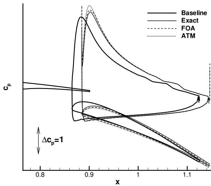
Figure 15. Baseline and optimized geometries and pressure distributions for the flap of the high-lift configuration, from optimizations performed with a variety of approximate discrete adjoint gradients. The results for TSL, CCA and CEV optimizations are not shown as they are indistinguishable from the exact optimization result.
