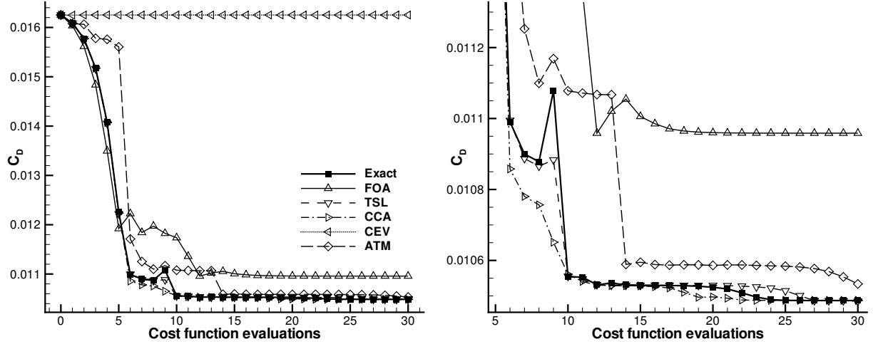
Figure 8. Convergence of the Quasi-Newton Trust Region method for drag minimization of the RAE2822 at constant lift. The optimization problem statement is identical to that of Fig. 4. Convergence is plotted for the method with various adjoint gradient approximations. As before the plot on the right shows details of the plot on the left near the optimum solution.
