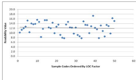
Figure 6. CRT Value for 50 Java Codes Ordered by LOC
