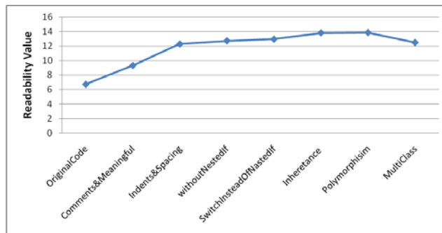
Figure 5. (DateAndTimeUtility.java) Readability Values
