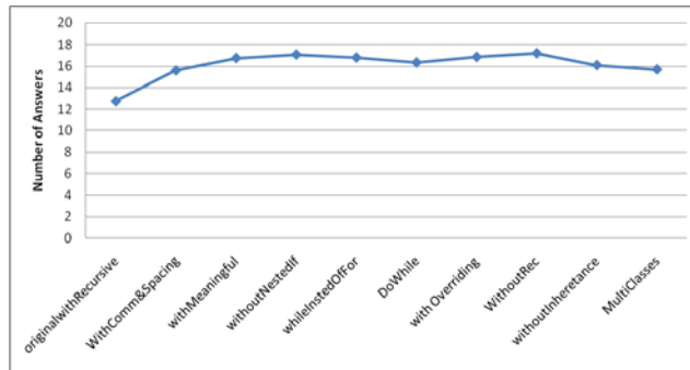
Figure 4. (Sudoku.java) Readability Values
