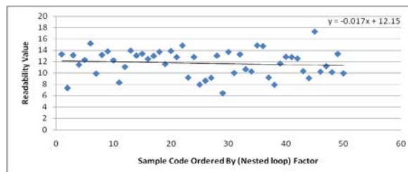
Figure 9. CRT Value for Codes Sample Ordered by (Nested Loop) Factor
