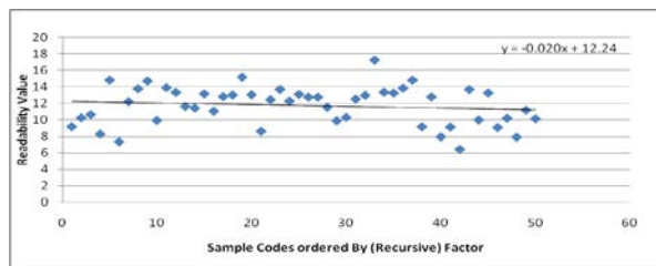
Figure 10. CRT Value for Codes Sample Ordered by (Recursive) Factor
