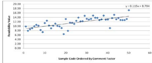
Figure 8. CRT Value for Codes Sample Ordered by (Comments) Factor
