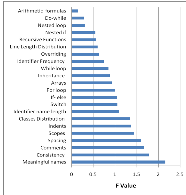
Figure 2. ANOVA Test (F) Measure for Factors with Experience and Job
