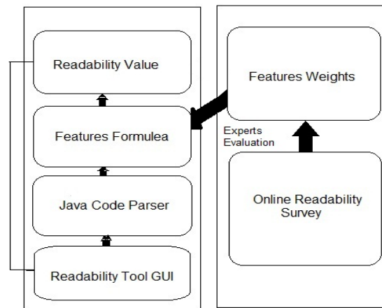
Figure 1. IPFCR Approach Workflow
