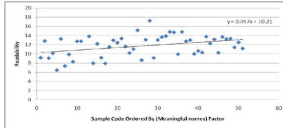
Figure 7. CRT Value for Codes Sample Ordered by (Meaningful Names)
