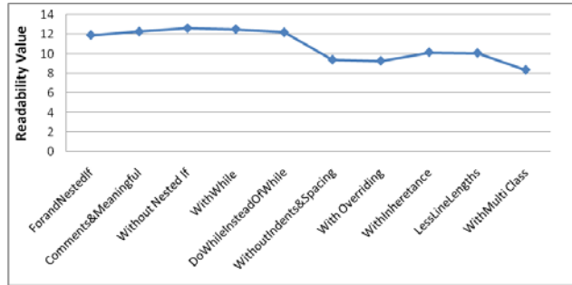
Figure 3. (Dijkstra.java) Readability Values
