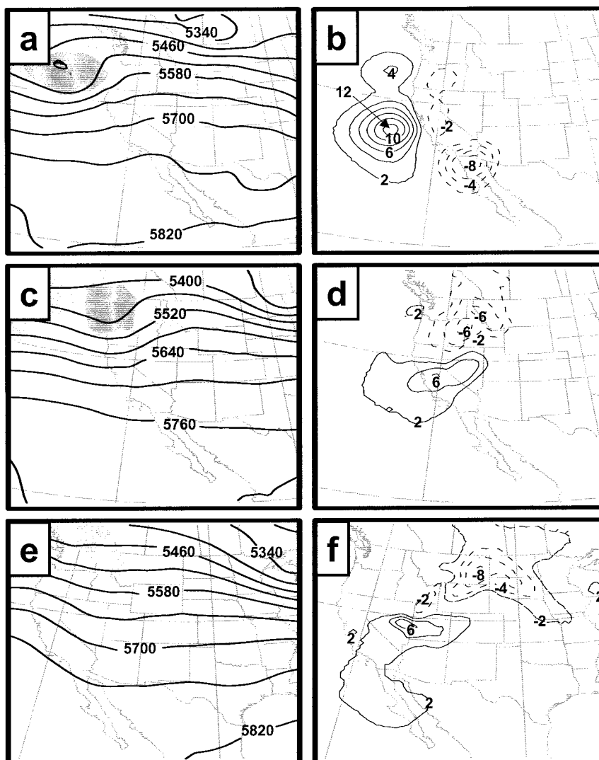
FIG. 2. Analyses of 500-mb height (m, solid) and sea level pressure (contours below 1008 mb shaded with 4-mb increments) during IOP-3 at (a) 0000 UTC 20 Feb, (c) 1200 UTC 20 Feb, and (e) 0000 UTC 21 Feb 1992. Increments (m, 2-m contour, solid positive, dashed negative) of 500-mb heights defined as the experiment–control forecast differences in (b), (d), and (f) that correspond to the times in (a), (c), and (e), respectively.
