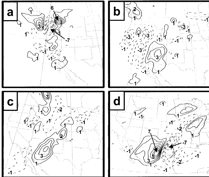
FIG. 5. Meridional wind increments ( \text{m s}^{-1} , 1 \text{ m s}^{-1} interval, dashed negative) at 500 mb defined as experiment–control during IOP-3 at (a) initial time of 0000 UTC 21 Feb and Eta forecasts after (b) 12, (c) 24, and (d) 48 h. Panel (c) corresponds to (c) and (d) in Fig. 4, and panel (d) corresponds to (e) and (f) in Fig. 4.
