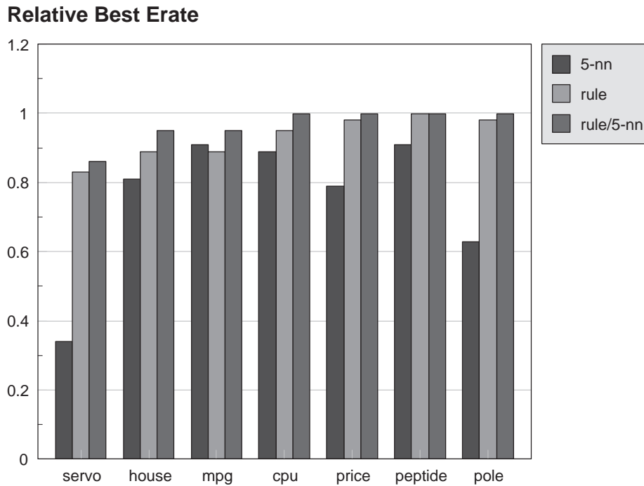
Figure 7: Relative Best Erates of 5-nn, Rules, and Rule/5-nn
