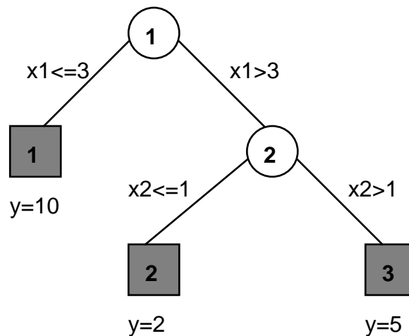
Figure 1: Example of Regression Tree
