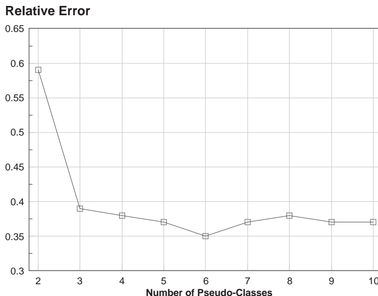
Figure 6: Prototypical Performance for Varying Pseudo-Classes
