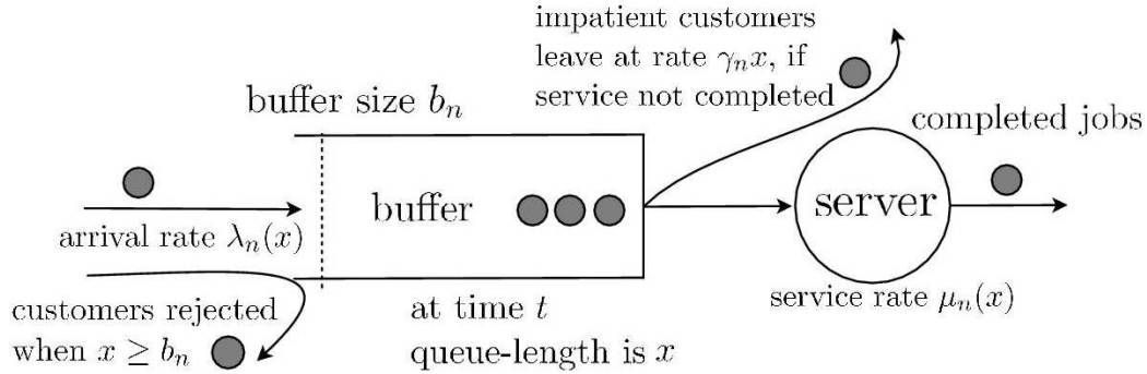
Figure 1: Dynamics of the n -th queueing system
