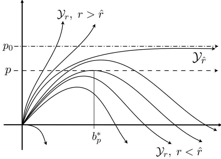
Figure 2: Nature of the family of solutions \mathcal{Y}_r
