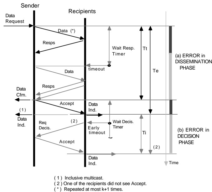
Figure 1: Timing diagram of AMP: In grey, in both phases, a transient omission error: a) Dissemination; b) Decision.
