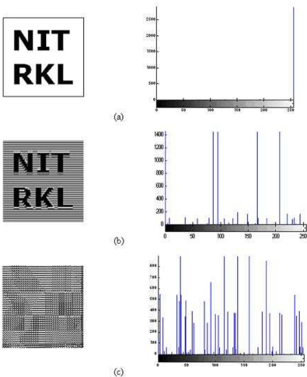
Figure 3.8: Histograms of (a) original nitrkl image (b) nitrkl image encrypted by original Hill cipher and (c) nitrkl image encrypted by AdvHill cipher
