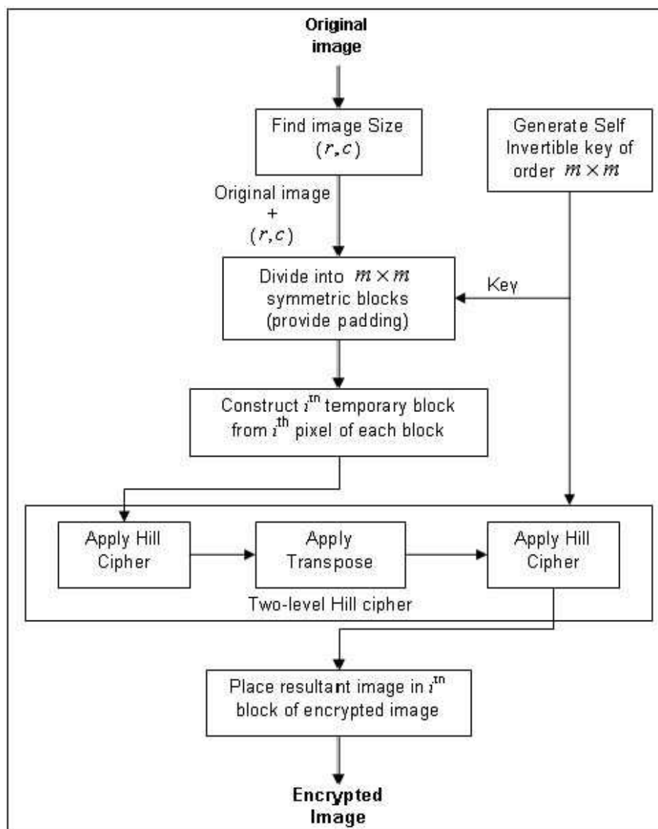
Figure 3.5: Block Diagram for proposed AdvHill Cipher Encryption
