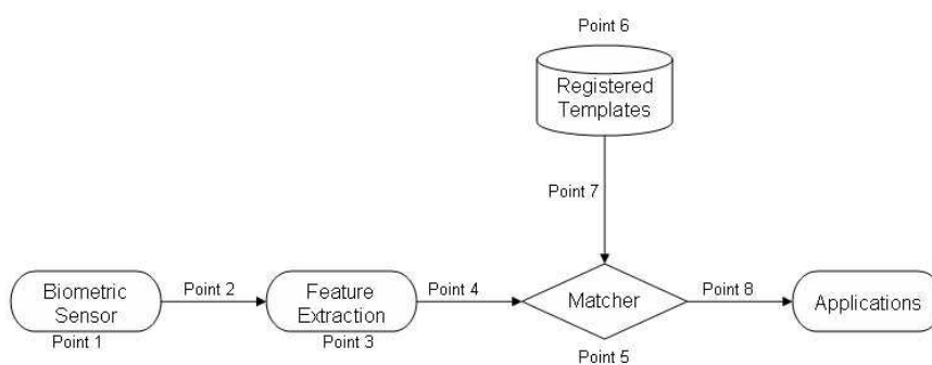
Figure 2.5: Potential attack points in a biometric system
