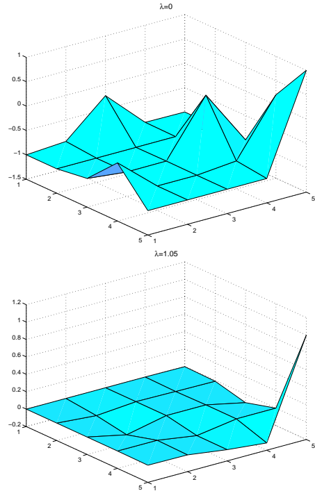
Figure 2. Inverse RL on the 5 \times 5 grid. Top: \lambda = 0 . Bottom: \lambda = 1.05 .
