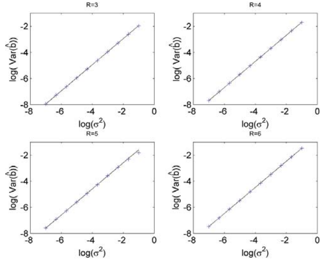
Fig. 3. MSEs of the MLE (blue crosses) for the nonlinearity parameter b and R = 3, 4, 5, 6 versus \sigma^2 compared with the CCRLBs (black lines).
