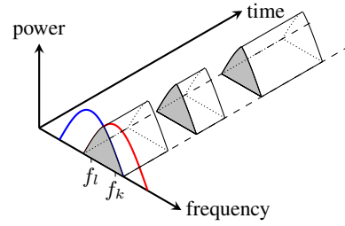
Fig. 1: The interference I_l(k) (Eq. (1)) can be seen as the average sum of the volumes spanned by the channel overlaps over time. The time intervals without volume correspond to the intervals during which k is idle.
