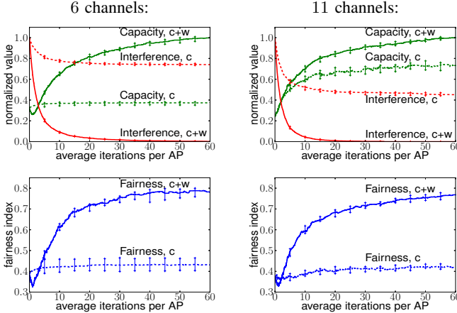
Fig. 4: Capacity, interference and fairness as functions of the number of iterations. We show the values obtained when SAW tunes both the channel center frequency and bandwidth ( c+w ), and when it tunes only the center frequency ( c ).
