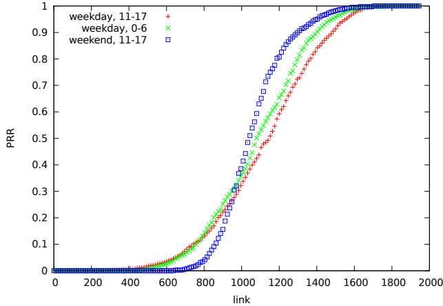
Figure 5. Mean PRR for different times of day.
