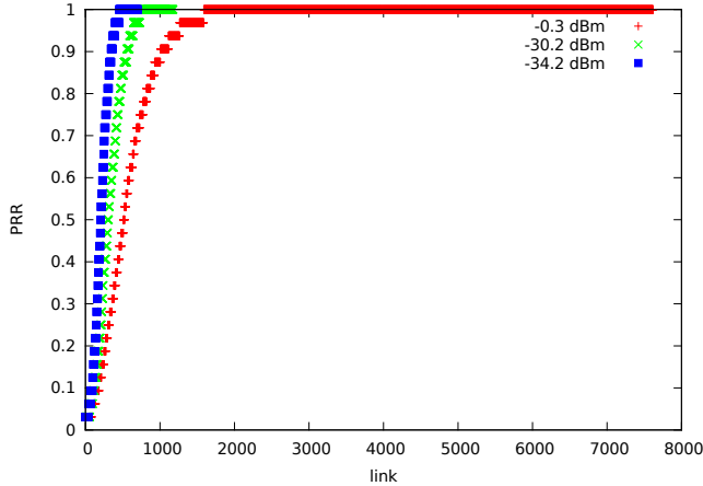
Figure 2. Distribution of the PRR at -0.3 dBm, -30.2 dBm and -34.2 dBm.
