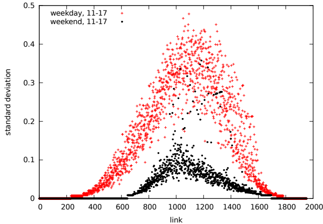
Figure 6. Standard deviation of PRR for different times of day.
