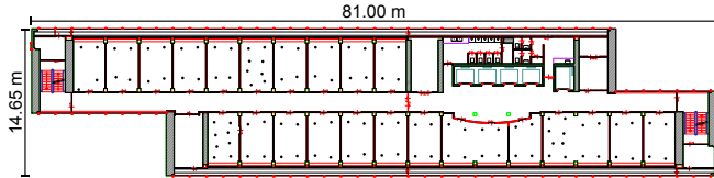
Figure 1. Floor plan of the 9th floor of the EEMCS building. The black dots indicate the locations of the 4 (or 8) nodes per room.
