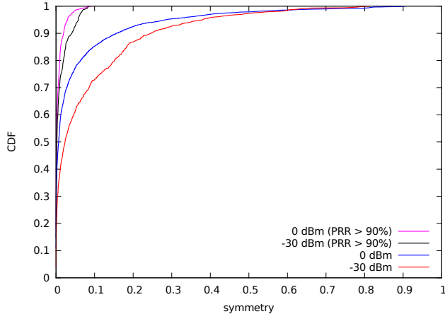
Figure 10. Distribution of the symmetry of the links
