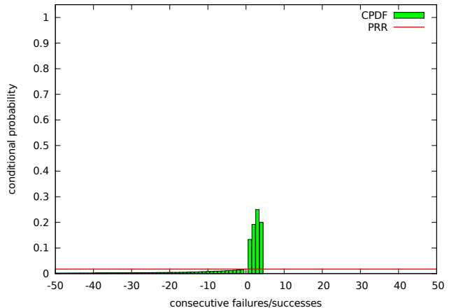
Figure 9. CPDF of link from node 56 to node 76 during a week day.
