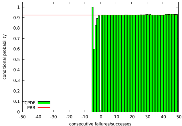
Figure 8. CPDF of link from node 56 to node 76 in a week night.
