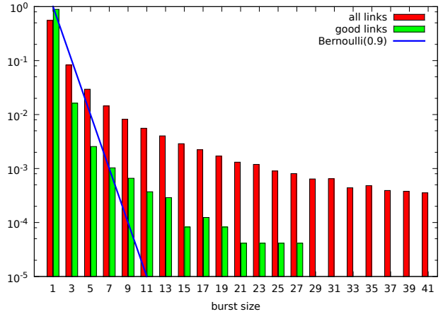
Figure 7. Burst errors for all and good links on a log scale.
