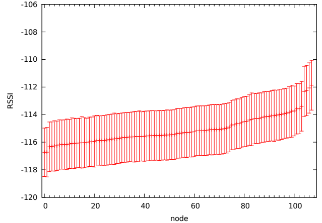
Figure 3. Ambient noise measurements on our testbed measured for 24 hours at 2 Hz during the week.
