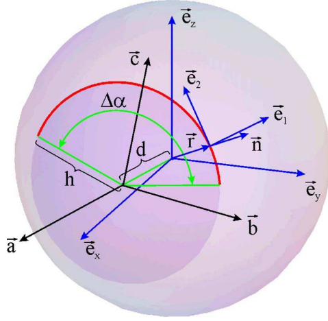
Figure 3: String reconstruction from sine-Gordon. The global coordinate system is defined by the constant basis vectors \{\vec{e}_x, \vec{e}_y, \vec{e}_z\} . The position of the string in space-time is expressed in the time-dependent basis \{\vec{a}, \vec{b}, \vec{c}\} . The trihedron \{\vec{e}_1, \vec{e}_2, \vec{n}\} is a set of basis vectors along the string.
