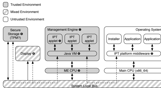
Figure 2: IPT abstract architecture (for a detailed explanation see §2.1.1)
