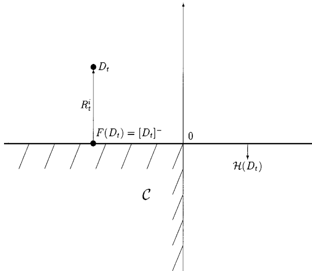
FIGURE 2.—Approaching \mathcal{E} = \mathbb{R}^L_- .
