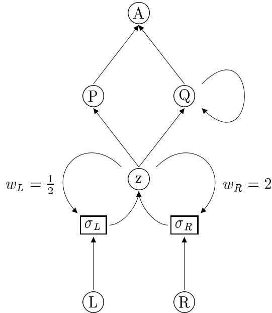
Figure 2: A neural network for parenthesis balancing.
