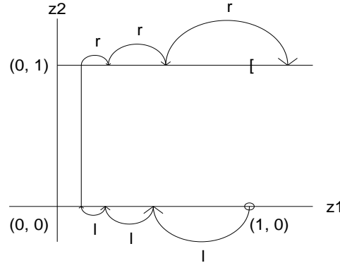
Figure 6: \mathcal{M}(1/2, 17/8) accepting l^3r^3 .
