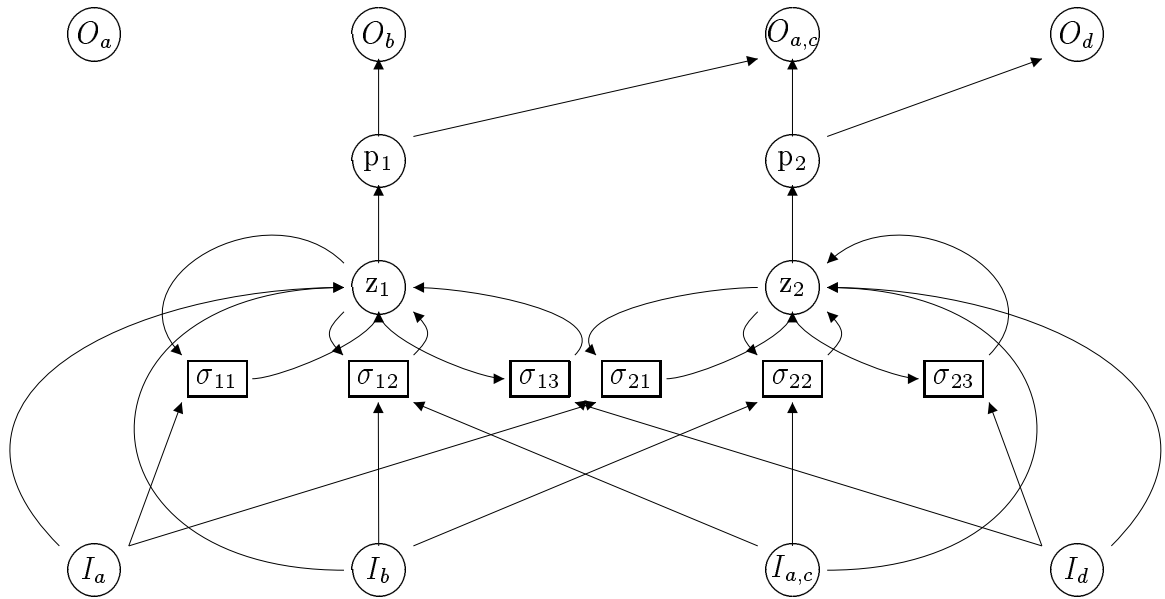
Figure 5: Network 1. A neural implementation of Grammar 1. Square nodes denote gating units and circular nodes denote signalling units.
