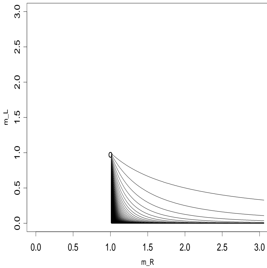
Figure 7: The bands in the space m_L \times m_R where the simplest (two-rule) context free languages reside. (Example 4.2).
