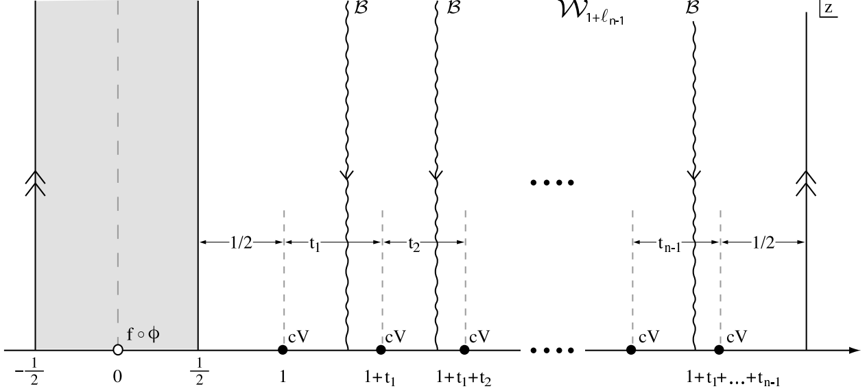
Figure 1: The surface \mathcal{W}_{1+l_{n-1}} with the operator insertions used to construct the solution \Psi^{(n)} given in (3.3). The parameters t_1, t_2, \dots, t_{n-1} must all be integrated from zero to one. The leftmost and rightmost vertical lines with double arrows are identified.
