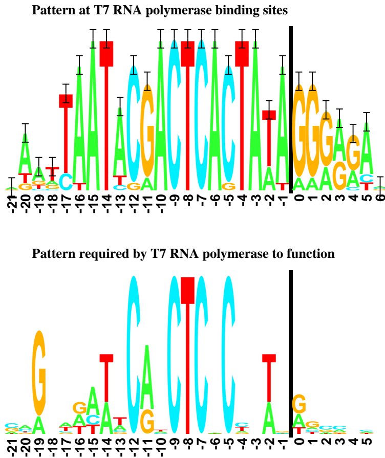
Figure 3: Logo for sequences at T7 RNA polymerase binding sites in the bacteriophage T7 genome (upper logo) and logo for the pattern that is required for T7 RNA polymerase alone to function (lower logo).
