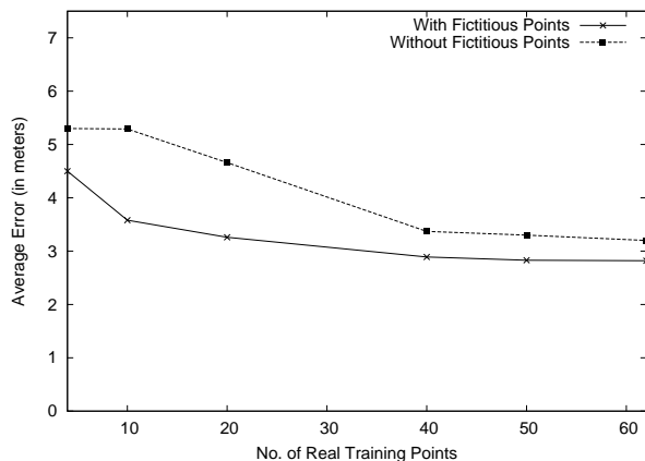
(a) KNN's performance with and without fictitious points
