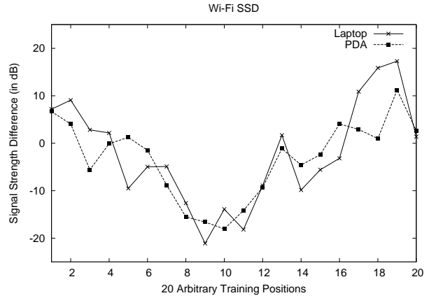
(d) Signal Strength Difference between 2 Wi-Fi APs
