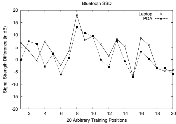
(c) Signal Strength Difference between 2 Bluetooth APs
