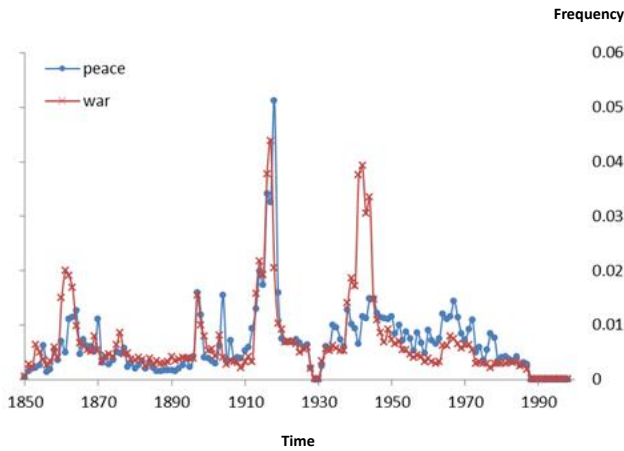
Figure 1: Time series (1870-1988) of the words “war” (red) and “peace”(blue). The words correlate over time.
