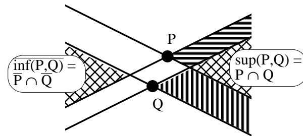
Fig. 18. Lattice structure of light cones
