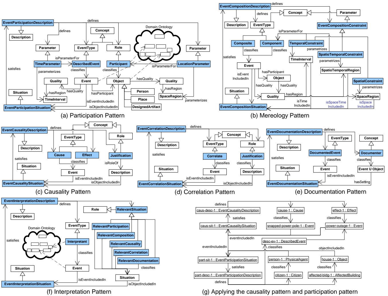
Figure 2: The patterns of F, namely (a) participation, (b) mereology, (c) causality, (d) correlation, (e) documentation, and (f) interpretation and (g) example of applying the F ontology
