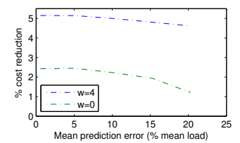
Fig. 4. Impact of prediction error on the Hotmail workload.
