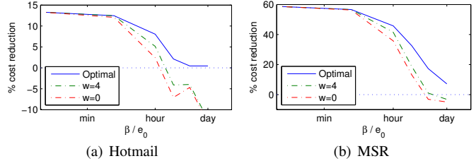
Fig. 8. Impact of switching cost, against time on a logarithmic scale.
