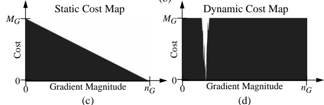
Figure 4: Comparison of live-wire (a) without and (b) with dynamic training. (a) Without training, the live-wire segment snaps to nearby strong edges. (b) With training, it favors edges with similar characteristics as those just learned. (c) The static gradient magnitude cost map shows that without training, high gradients are favored since they map to low costs. However, with training, the dynamic cost map (d) favors gradients similar to those sampled from the previous boundary segment.
