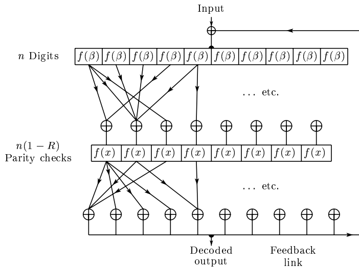
Figure 4.2: Decoding apparatus
