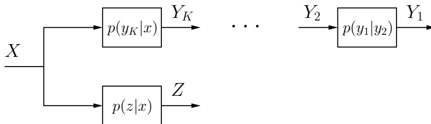
Figure 2: The degraded multi-receiver wiretap channel with a more noisy eavesdropper.
