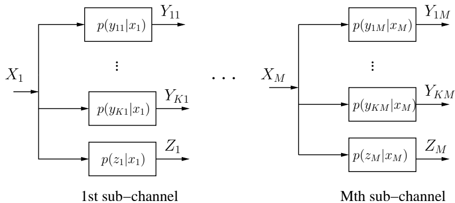
Figure 3: The parallel multi-receiver wiretap channel.
