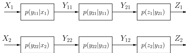
Figure 4: The parallel degraded multi-receiver wiretap channel.
