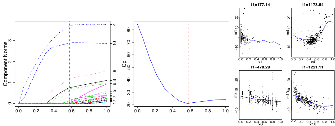
Figure 3: (Boston housing) Left: The empirical \ell_2 norm of the estimated components versus the regularization parameter \lambda . Center: The C_p scores against \lambda ; the dashed vertical line corresponds to best C_p score. Right: Additive fits for four relevant variables.
