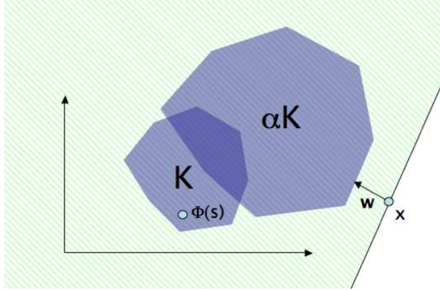
FIG. 3.2. An approximation algorithm run on vector w \in \mathcal{W} always returns a point s \in \mathcal{S} such that the set \alpha K is contained in the halfspace tangent to \Phi(s) whose normal direction is w . An extended approximation algorithm, as illustrated here, takes any w \in \mathbb{R}^n as input and returns a point x \in \mathbb{R}^n such that \alpha K is contained in the halfspace tangent to x with normal vector w . In addition, it returns an s \in \mathcal{S} such that \Phi(s) dominates x .
