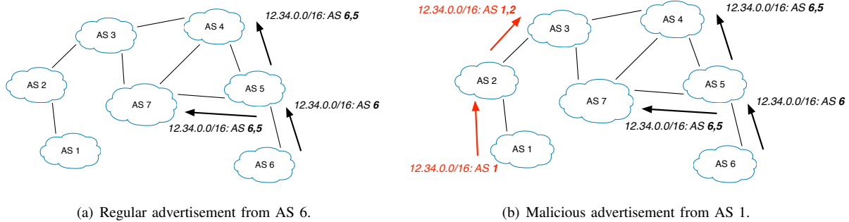
Fig. 2. Announcement of prefix 12.34.0.0/16 originating from the valid AS 6 and from a malicious AS 1. AS 2 and 3 will prefer the malicious advertisement from AS 1 because the path length will be shorter than the valid advertisements from AS 6.
