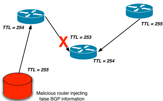
Fig. 4. The Generalized TTL Security Mechanism (GTSM) in operation. Routers set the TTL on a packet to 255, which is decremented when it reaches the peer. If the router is configured such that no packets with a TTL of less than 254 will be accepted, then remote adversaries attempting to inject malicious information to a router will have their packets dropped.
