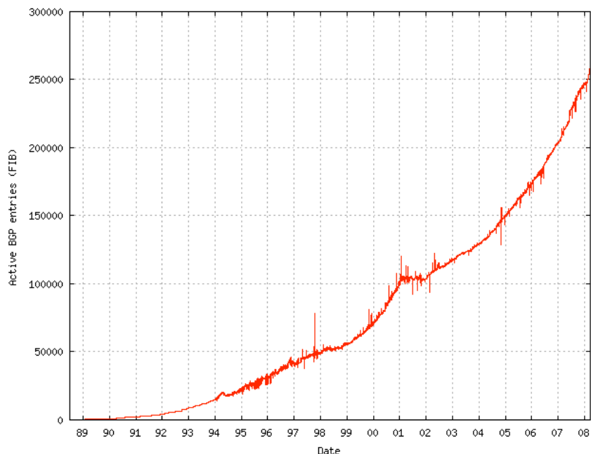
Fig. 7. 1988-2008 routing table updates from the CIDR report ( http://www.cidr-report.org/ )
