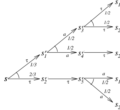
Fig. 3: A representation of a weak transition with action a .
