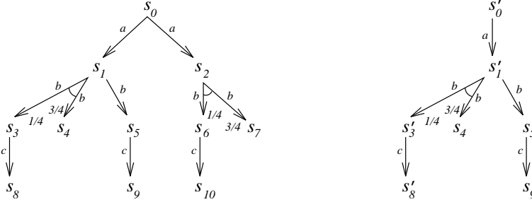
Fig. 1: Strong simulations do not preserve EU_{\geq p} .
