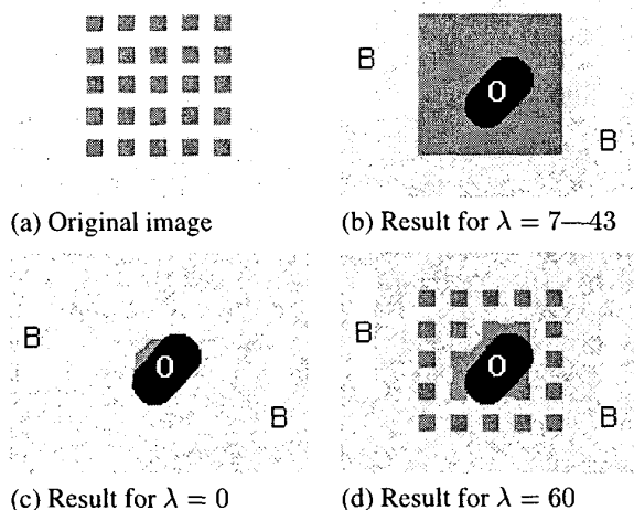
Figure 2. Synthetic Gestalt example. The segmentation results in (b-d) are shown for various levels \lambda of relative importance of “region” versus “boundary” in (1). Note that the result in (b) corresponds to a wide range of \lambda .
