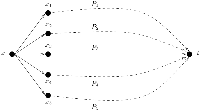
Fig. 4. The second type of move tries to make all paths from n to t of equal length.
