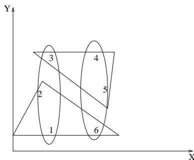
Fig. 24. The leader algorithm is order dependent.
