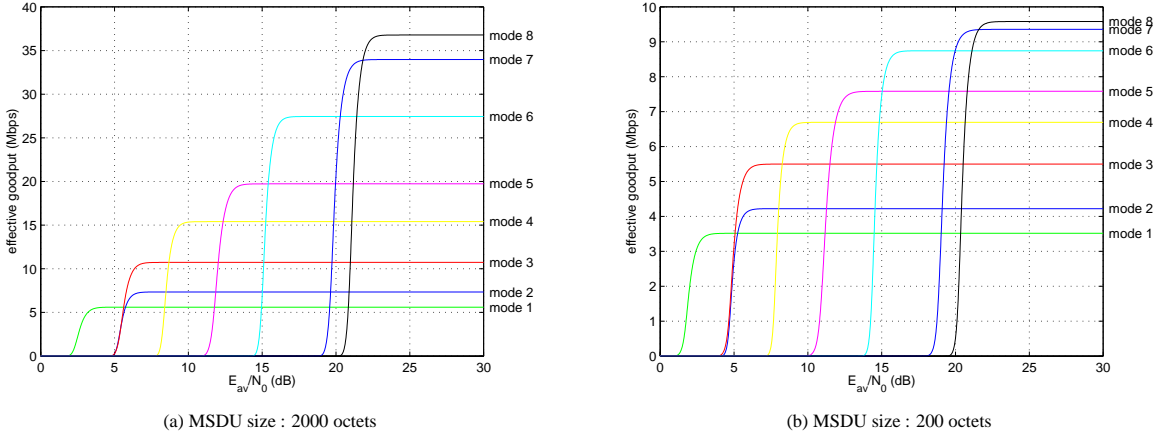
Fig. 7. Effective Goodput vs. SNR
