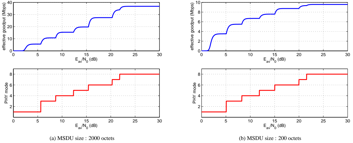
Fig. 8. MSDU-based adaptive PHY mode selection to improve the effective goodput
