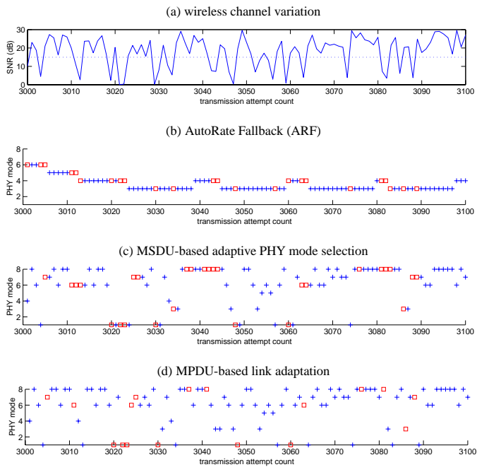
Fig. 15. Adaptability comparison of three link adaptation schemes
