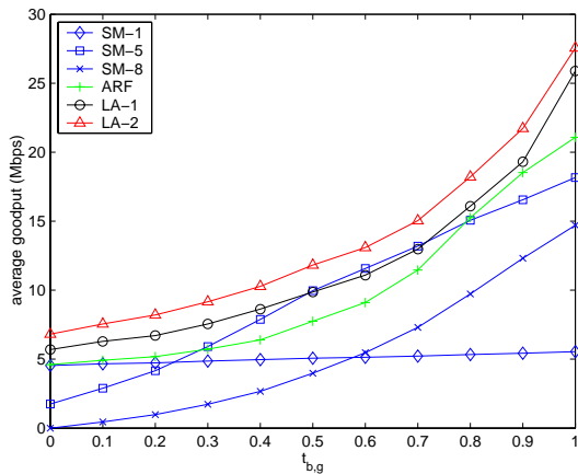
Fig. 14. Goodput comparison of the testing schemes
