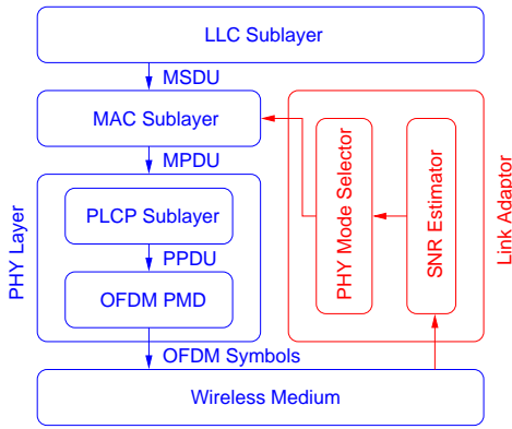
Fig. 10. System architecture for link adaptation
